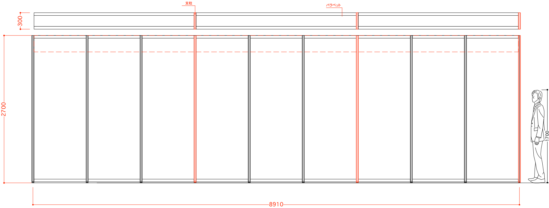
■ A-elevation
