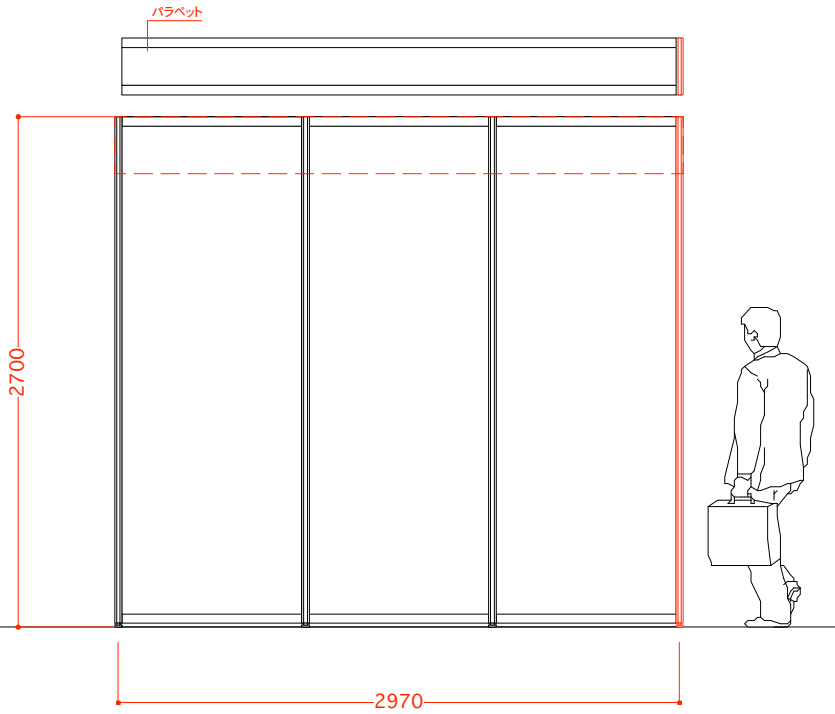
■ B-elevation
