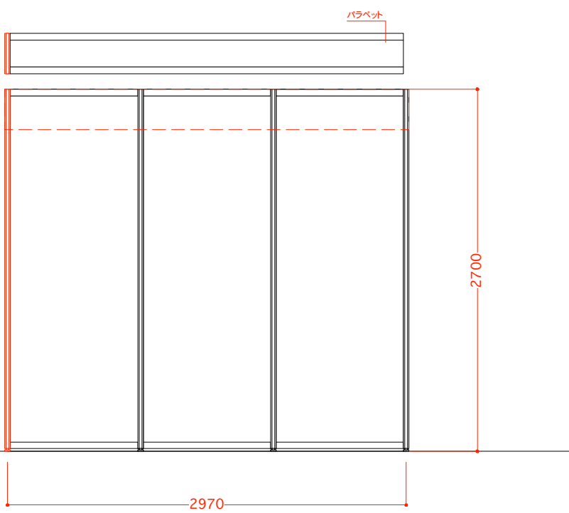
■ B-elevation
