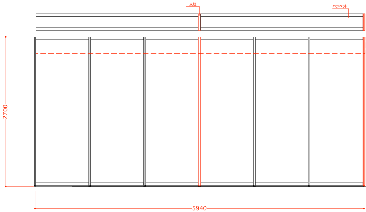
■ A-elevation
