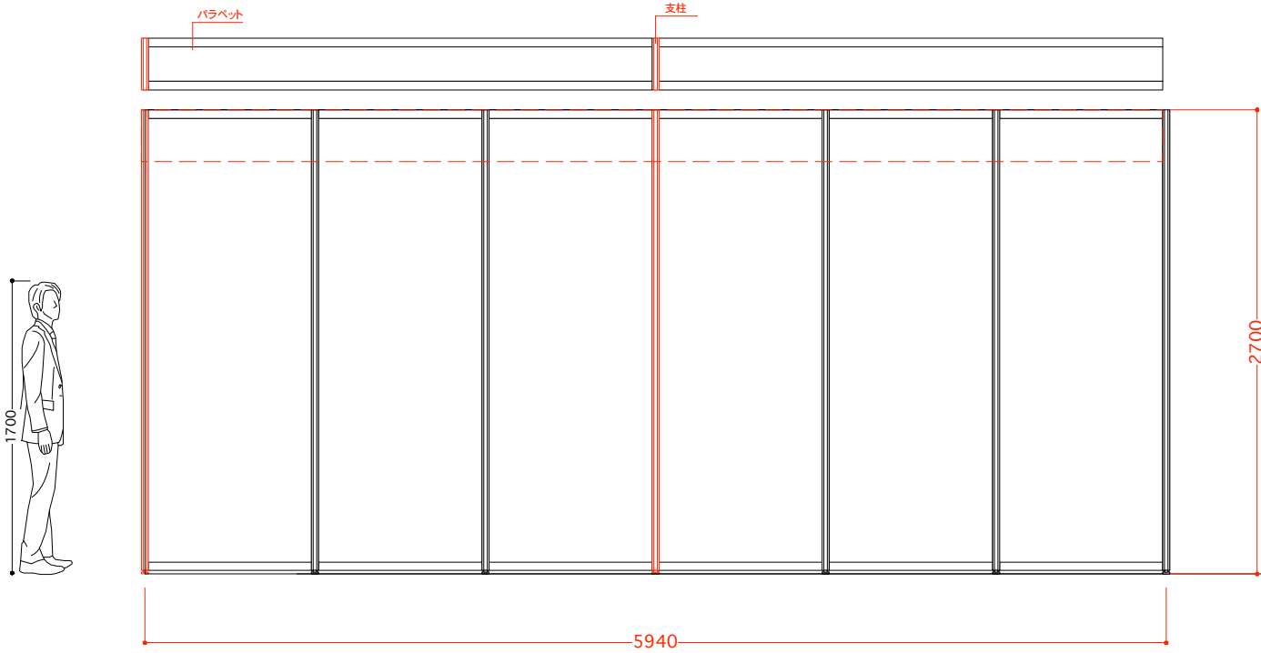
■ A-elevation
